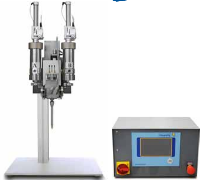
Feeding and Metering Unit: Dos A90 + SCP 200 (switch cabinet)
